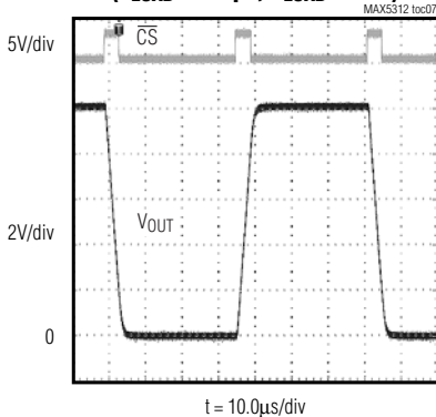
UNIPOLAR SETTLING TIME ( C_{LOAD} = 250pF , R_{LOAD} = 2k\Omega )
