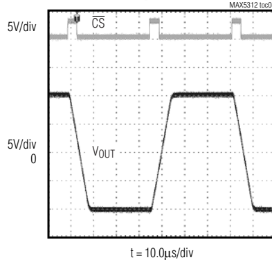
BIPOLAR SETTLING TIME ( C_{LOAD} = 250pF , R_{LOAD} = 10k\Omega )
